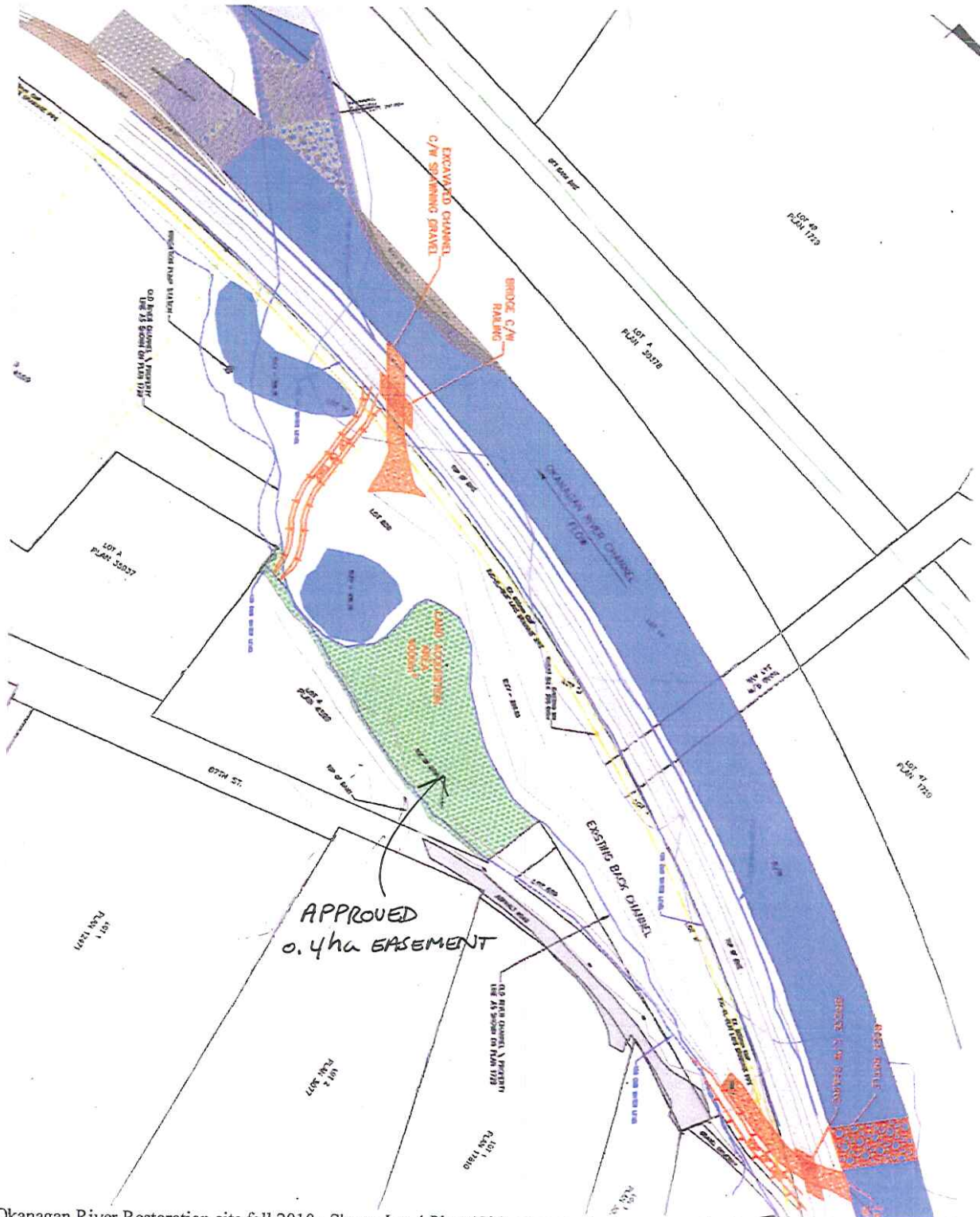
Figure #1 Engineers Diagram ORRI Phase II
